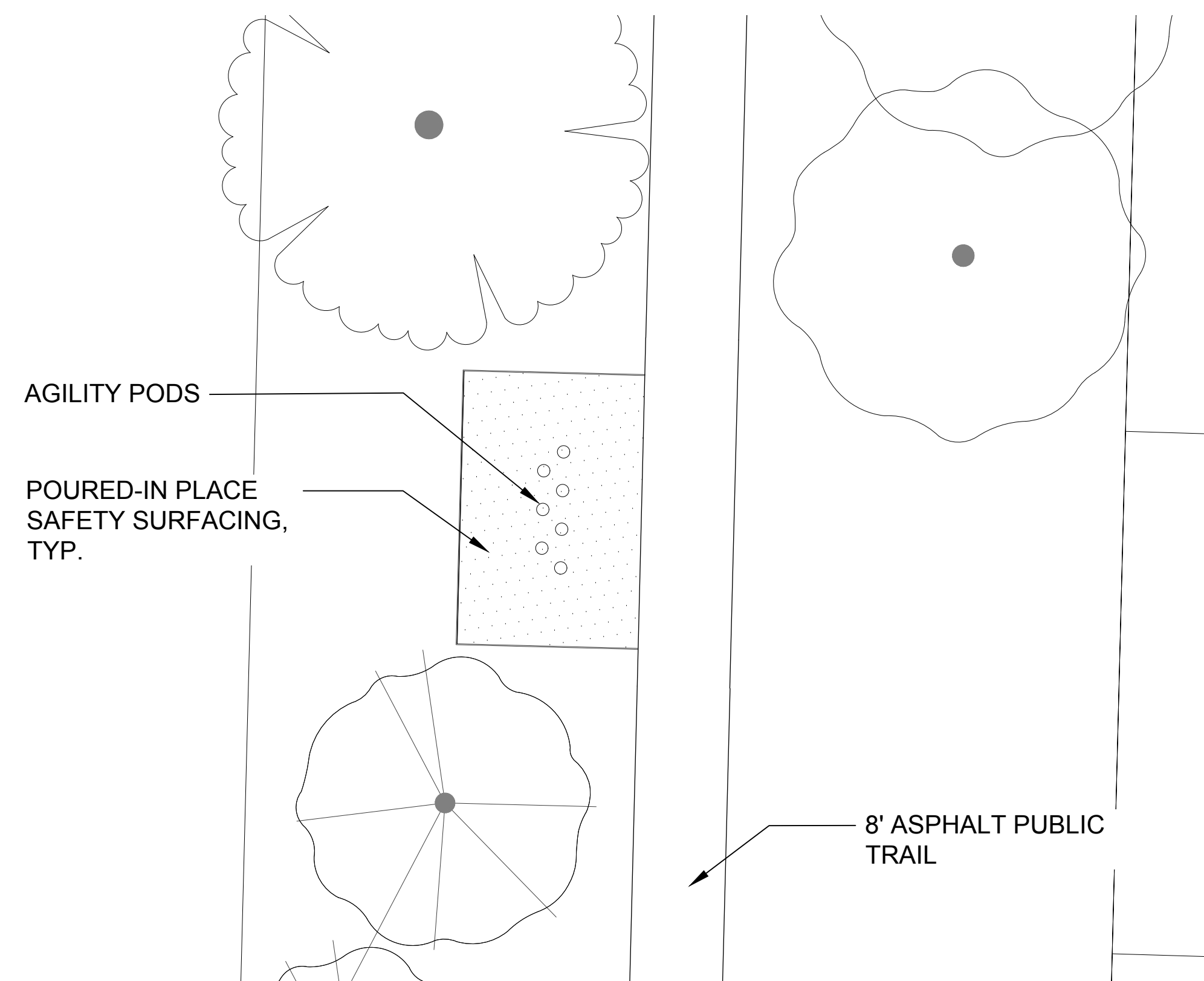
B FITNESS STATION ENLARGEMENT
