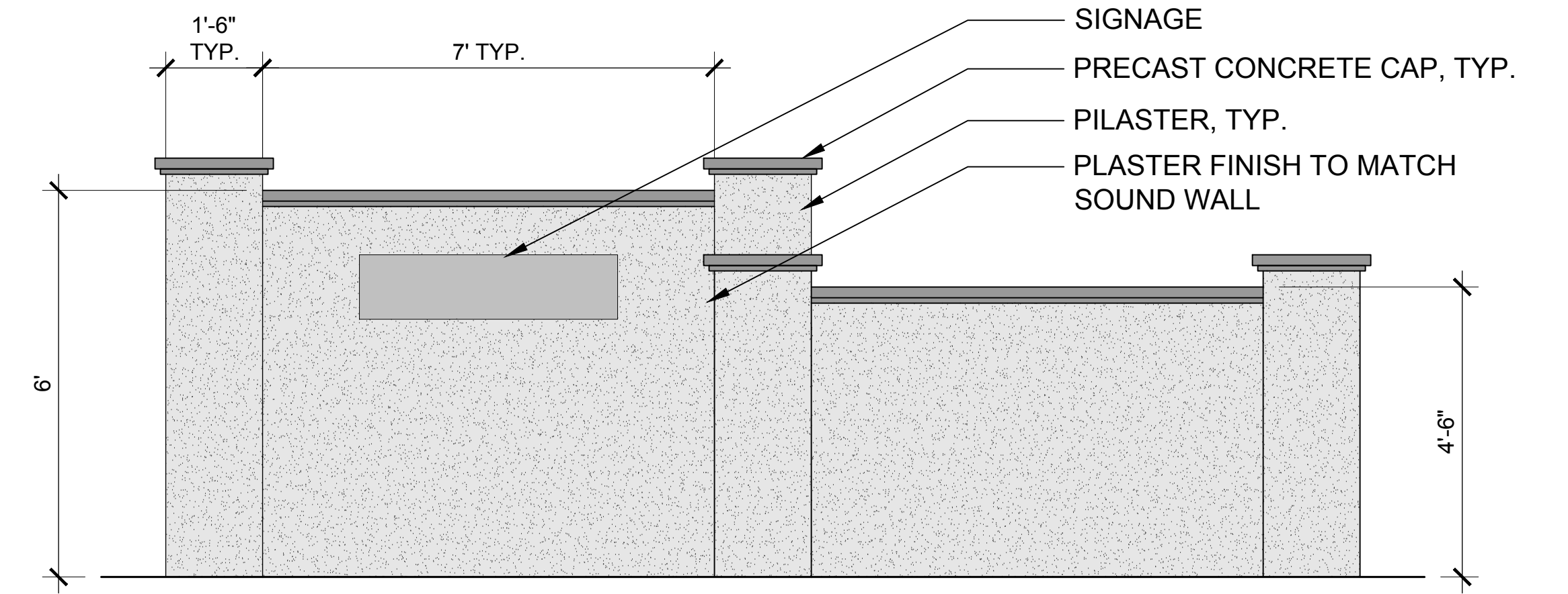
ENTRY MONUMENT WALL
