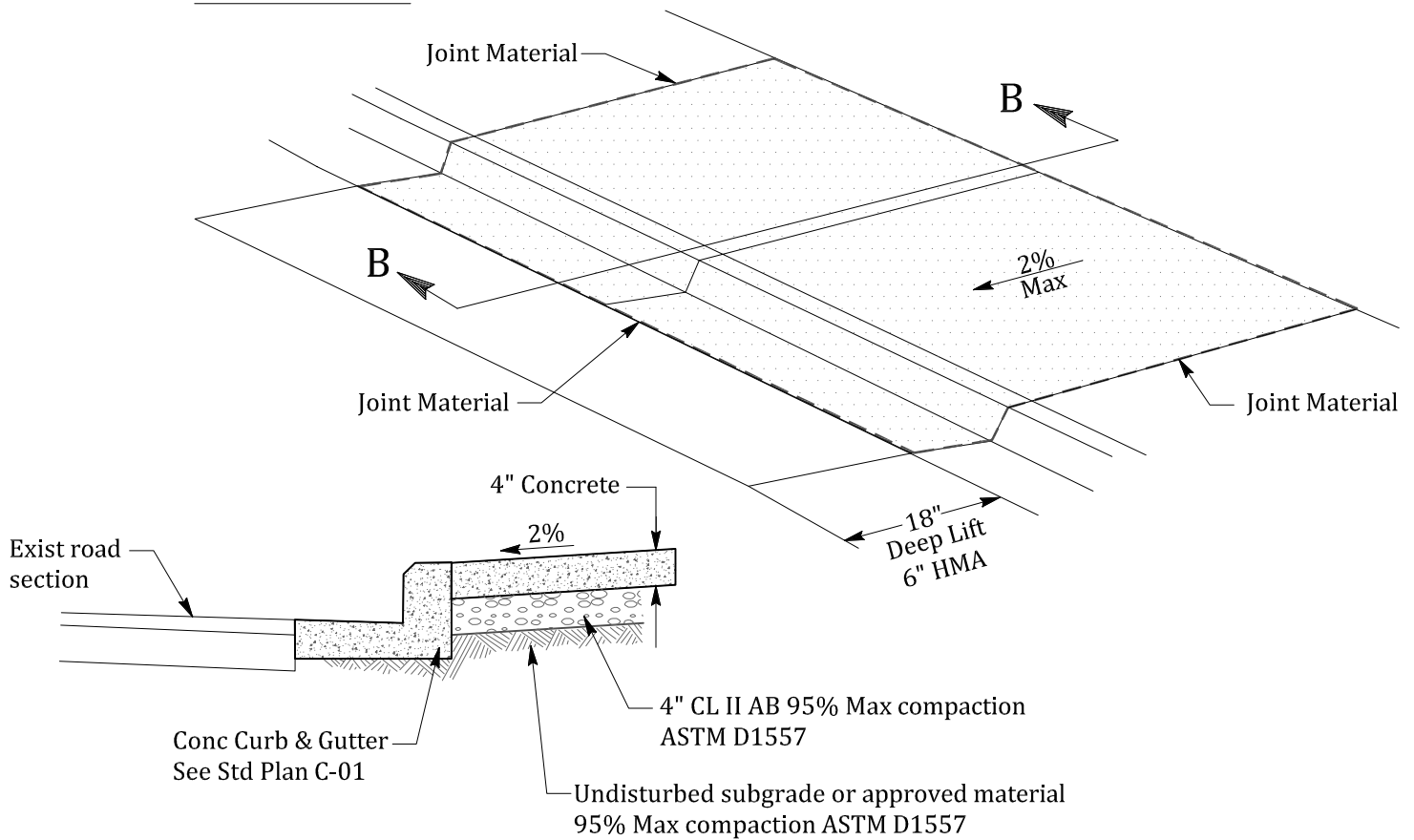
SECTION B-B
